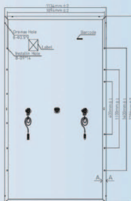
Back View
