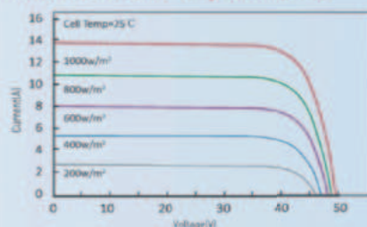
I-V/P-V Curve at Different Irradiation (585W)
