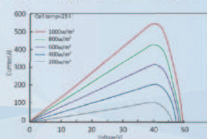
I-V/P-V Curve at Different Irradiation (585W)
